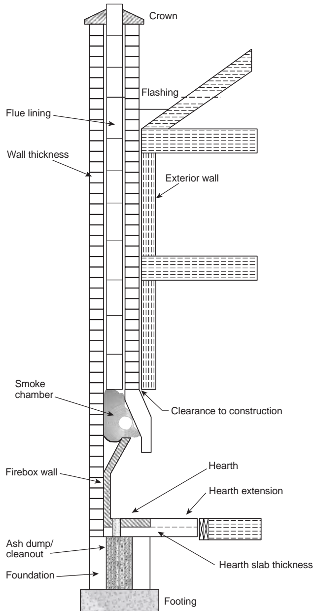
FIGURE A.11.2(a) Fireplaces and Chimney Details.
